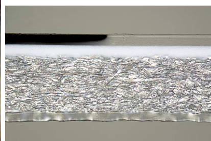
Figures 99 and 100 – Inkjet print (dye) on a swellable support. Cross-section at 200x with BF reflected light and DF-UV light (left to right). The RC backing and front layer cause this fluorescence.
