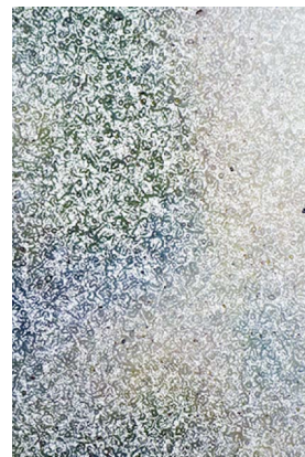
Figures 59 and 60 – Carbro. 50x view at 45° and 0° lighting (left to right). At 45° it is possible to observe pigment particles and missregistration between the blue and yellow layers. At 0° the image shows differential gloss.
