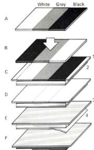
Figure 144 – The carbro process. It is distinguished from the carbon process because the negative is printed on B&W silver bromide paper, and this bromide is squeezed against carbon tissue. The bleaching of the silver image will provoke selective hardening of the tissue. It is then placed on a temporary support, washed and the relief image is transferred to the final support. In Coe, 98.
