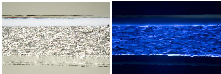
Figures 73 and 74 – Cibachrome print. Cross section at 200x view, with BF reflected light and DF-UV light (left to right). A fiber based core is in between two RC coatings, which is shown by the fluorescence. The dye layers are over a white pigmented RC layer for more contrast.
